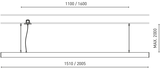
LINE SUSPENSION D&I 1500 / 2000
