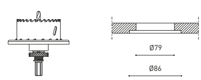
TRIMLESS TOOL D79 X D86mm A478-00-04
