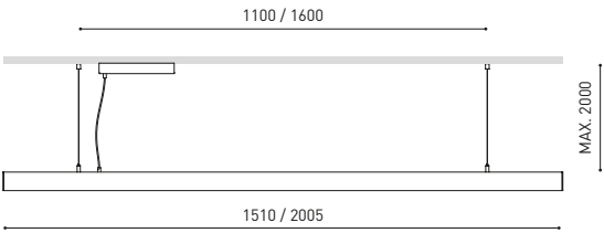
LINE SUSPENSION D&I 1500 BASE / 2000 BASE
