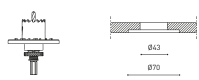
TRIMLESS TOOL D43 X D70mm A478-00-02
