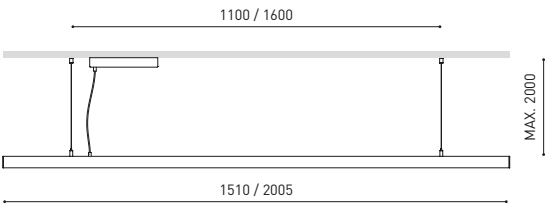
LINE SUSPENSION 1500 BASE / 2000 BASE
